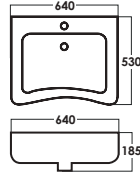
SRTWB246 D: L640xW530xH185mm (Included Fixing Bolt)
