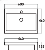
SRTWB7098 D: L600xW460xH155mm
