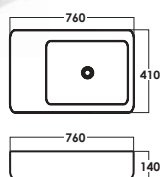
SRTWB1541 D: L760xW410xH140mm LP: RM 950
