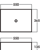
SRTWB3418 D: L550xW365xH135mm
