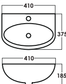
SRTWB245 D: L410xW375xH185mm (Included Fixing Bolt)
