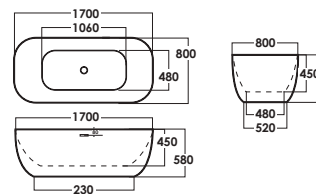
SRTBT1865-17 Free Standing Bathtub D: L1700xW800xH580mm Material : Acrylic LP: RM 7,764
