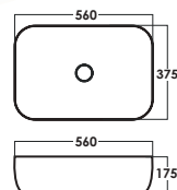
SRTWB7109-BL D: L560xW375xH175mm Black
