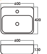
SRTWB1516-GY D: L600xW420xH130mm Golden Yellow
