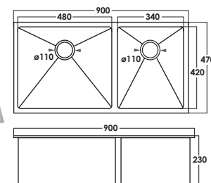
SRTKS7080 LP: RM 1,350 D: L900xW470xH230mm
