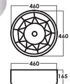
SRTWB3405 D: L460xW460xH165mm
