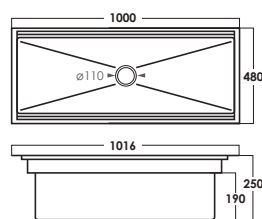
SRTKS1048-BL D: L1000xW480xH250 mm Matt Black
