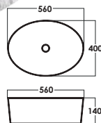
SRTWB3416 D: L560xW400xH140mm
