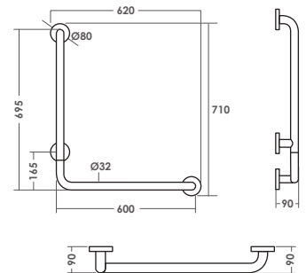
SRT5674 LP: RM 375 L620xW90xH710mm D: 32mm
