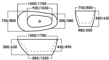
SRTBT1862-15 / 17 Free Standing Bathtub D: L1500xW750xH630mm (R) D: L1700xW800xH630mm (L) Material : Acrylic LP: RM 6,788 LP: RM 7,456
