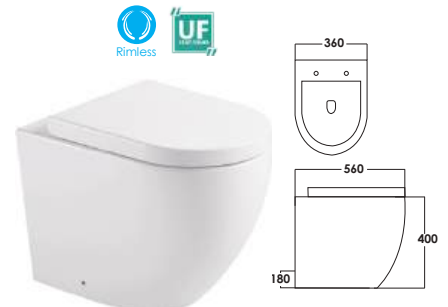
SRTWC6006-RL-UF Washdown Flushing Technology D : L560xW360xH400mm P-Trap : Horizontal Outlet 180mm *UF Seat Cover
