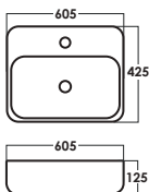
SRTWB1516-BW D: L605xW425xH125mm Black + White
