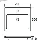
SRTWB2390 D: L900xW500xH210mm LP: RM 585
