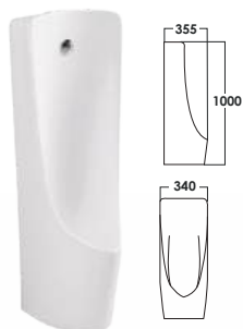
SRTUB6213 SRTUB6213-BI Floor Standing Urinal Bowl D : L355xW340xH1000mm Top Inlet / Back Inlet
