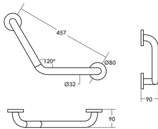
SRT393B-18 LP: RM 172 L457xW90mm D: 32mm
