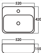
SRTWB1515-BW D: L520xW420xH155mm Black + White
