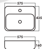
SRTWB7292 D: L575xW435xH160mm LP: RM 454
