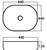
SRTWB1413-GW D: L440xW440xH135mm Golden Yellow + White
