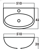
SRTWB243 D: L510xW420xH200mm (Included Fixing Bolt)
