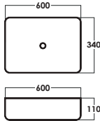
SRTWB3414-BW D: L600xW340xH110mm Black + White
