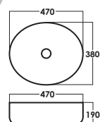
SRTWB7518 D: L470xW380xH190mm
