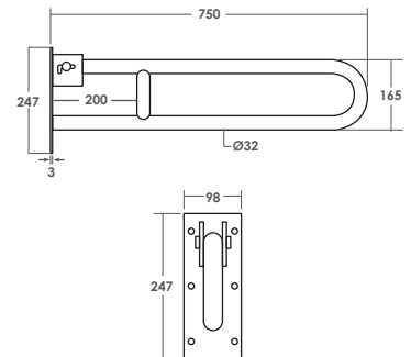
SRT5732 LP: RM 600 L750xW98xH247mm D: 32mm
