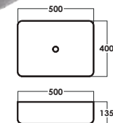
SRTWB3402 D: L500xW400xH135mm
