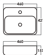
SRTWB1514-BL D: L460xW421xH157mm Black
