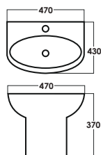
SRTWB5300 D: L470xW430xH370mm (Included Fixing Bolt)
