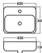
SRTWB248 D: L430xW360xH150mm (Included Fixing Bolt)
