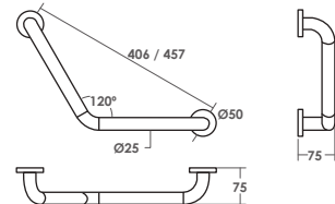
SRT393-16 LP: RM 115 L406xW75mm SRT393-18 LP: RM 119 L457xW75mm D: 25mm
