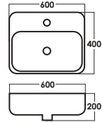
SRTWB888 D: L600xW400xH200mm (Included Fixing Bolt)
