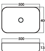
SRTWB1411-RG D: L500xW400xH135mm Rose Gold
