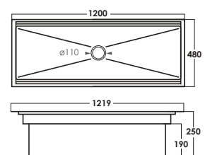
SRTKS1248-BL D: L1200xW480xH250mm Matt Black
