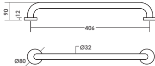
SRT392B-16 LP: RM 158 L406xW90xH80mm D: 32mm
