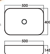
SRTWB1086-RG D: L500xW400xH145mm Rose Gold
