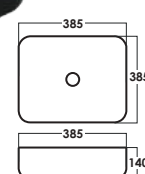
SRTWB1421-BW D: L385xW385xH140mm Black + White
