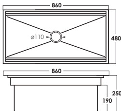
SRTKS8648-BL D: L860xW480xH250mm Matt Black
