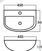
SRTWB D: L450xW365xH170mm (Included Fixing Bolt)
