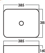
SRTWB1421-RW D: L385xW385xH140mm Rose Gold + White
