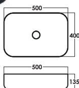
SRTWB1411-BL D: L500xW400xH135mm Black
