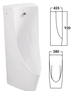
SRTUB905-BI Floor Standing Urinal Bowl c/w Sensor Flushing Fitting D : L425xW380xH920mm Back Inlet
