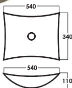
SRTWB3413-GY D: L540xW340xH110mm Gold
