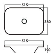
SRTWB1633 D: L515xW380xH190mm
