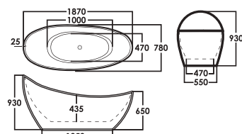
SRTBT1836 Free Standing Bathtub D: L1870xW780xH930mm Material : Acrylic LP: RM 9,284
