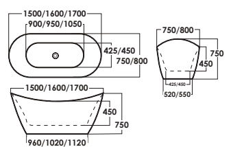
SRTBT1870-15 / 16 / 17 Free Standing Bathtub D: L1500xW750xH750mm (S) D: L1600xW800xH750mm (R) D: L1700xW800xH750mm (L) Material : Acrylic LP: RM 7,232 LP: RM 7,476 LP: RM 7,736
