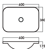
SRTWB1610 D: L600xW380xH175mm
