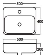
SRTWB890-BL D: L500xW400xH200mm Black (Included Fixing Bolt)
