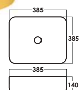
SRTWB1421-GY D: L385xW385xH140mm Golden Yellow
