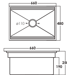
SRTKS6648-BL D: L660xW480xH250mm Matt Black
