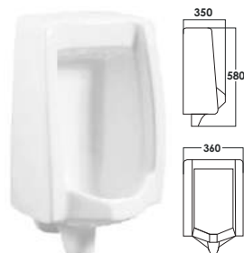
SRTUB5202 SRTUB5202-NZ Wall Hung Urinal Bowl D : L350xW360xH580mm Top Inlet / Nozzle
