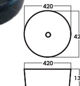
SRTWB3404 D: L420xW420xH135mm
