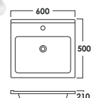
SRTWB2250 D: L600xW500xH210mm LP: RM 405
