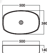
SRTWB1543 D: L500xW380xH140mm LP: RM 473
