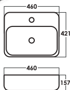
SRTWB1514-BW D: L460xW421xH157mm Black + White
