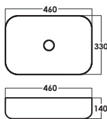
SRTWB2805-BL D: L460xW330xH140mm Black
