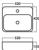
SRTWB1515-BL D: L520xW420xH155mm Black
