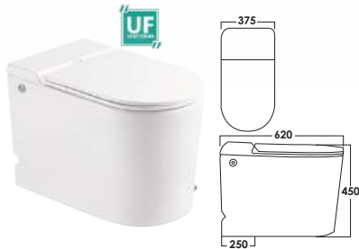
SRTWC8122 Electronic Pulse Water Closet Siphonic Flushing Technology D : L620xW375xH450mm S-Trap: Bottom Outlet 250mm *UF Seat Cover
