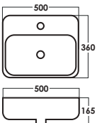
SRTWB247 D: L500xW360xH165mm (Included Fixing Bolt)
