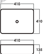
SRTWB3401 D: L410xW410xH135mm
