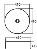
SRTWB7069 D: L410xW410xH165mm LP: RM 298
