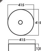
SRTWB1409-RB D: L415xW415xH135mm Black + Rose Gold
