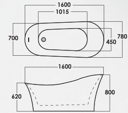
SRTBT1860-16 Free Standing Bathtub D: L1600xW780xH800mm Material : Acrylic LP: RM 7,588
