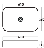
SRTWB1419 D: L610xW350xH115mm LP: RM 468
