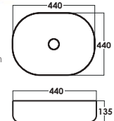
SRTWB1413-RW D: L440xW440xH135mm Rose Gold + White
