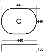
SRTWB1413-GY D: L440xW440xH135mm Golden Yellow
