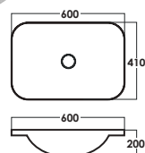
SRTWB1620 D: L600xW410xH200mm
