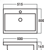
SRTWB7018 D: L515xW500xH165mm
