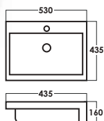
SRTWB7014 D: L530xW435xH160mm
