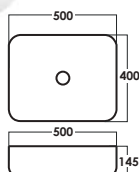
SRTWB1086 D: L500xW400xH145mm LP: RM 306
